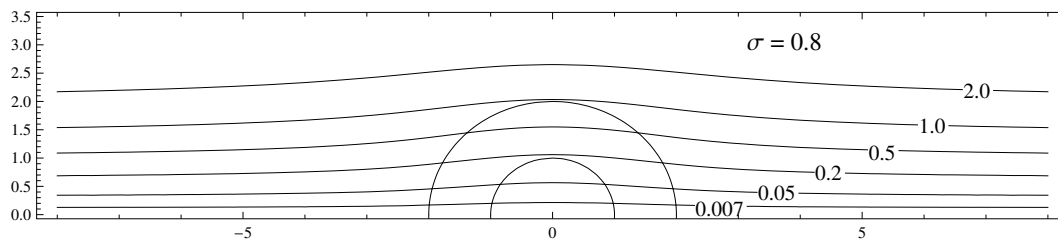
Figure 3. Stream lines \psi = c for c = 0.007, 0.05, 0.2, 0.5, 1.0, 2.0 when q = 2 and \sigma = 0.8
