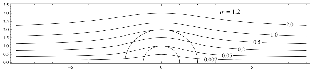
Figure 4. Stream lines \psi = c for c = 0.007, 0.05, 0.2, 0.5, 1.0, 2.0 when q = 2 and \sigma = 1.2
