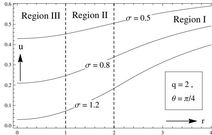
Figure 5. Variation of radial velocity u with radial distance r
