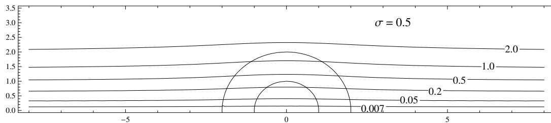
Figure 2. Stream lines \psi = c for c = 0.007, 0.05, 0.2, 0.5, 1.0, 2.0 when q = 2 and \sigma = 0.5
