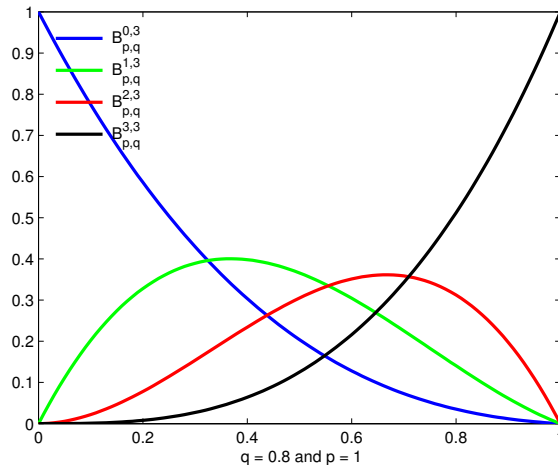
Figure 1. Cubic Bezier blending functions
