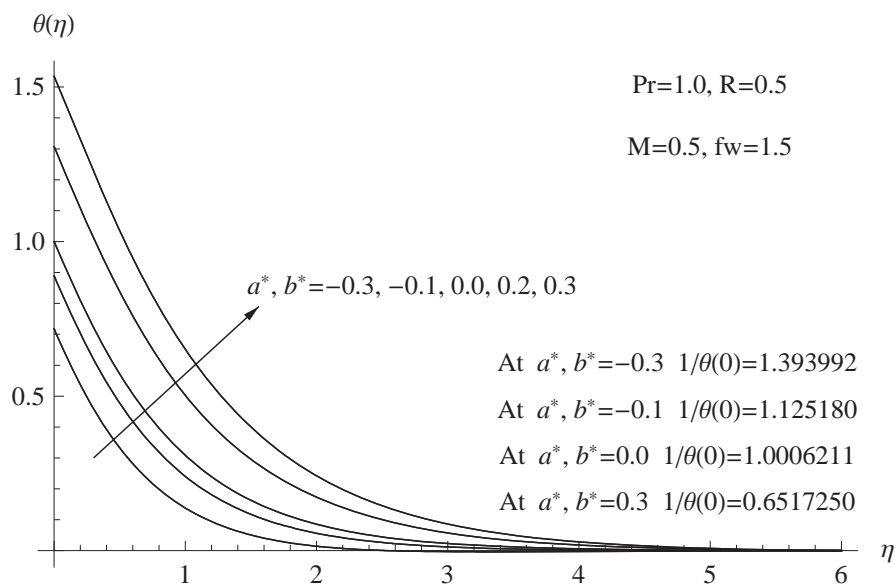
Figure 5. The behavior of the temperature distribution for various values of a^* and b^*
