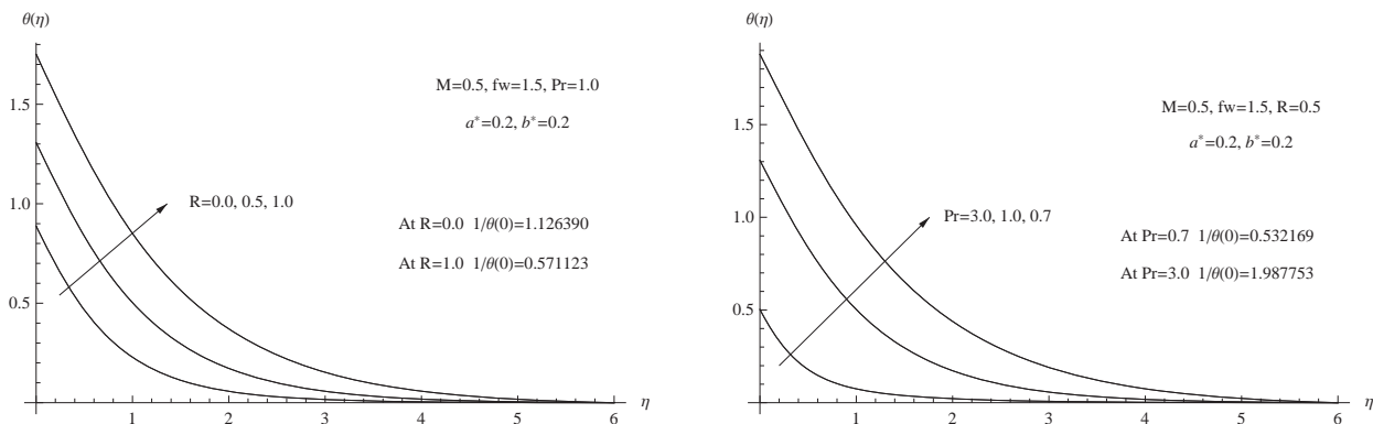
Figure 4. (a) Temperature distribution for R . (b) Temperature distribution for Pr
