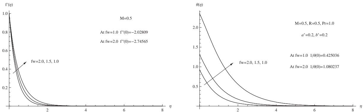
Figure 3. (a) Velocity distribution for f_w . (b) Temperature distribution for f_w
