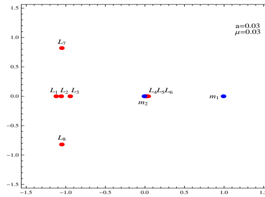
Figure 2. Location of non-collinear and collinear points
