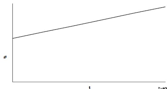
Figure 1. Higg's Field \phi Vs Time t
