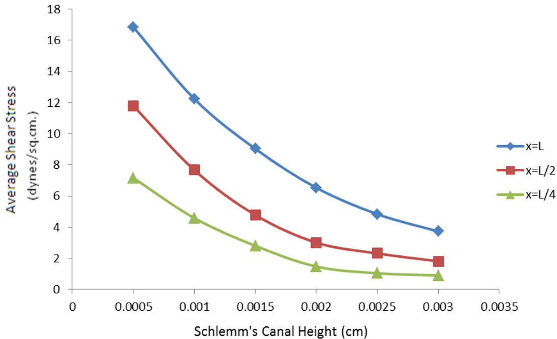
Figure 6. Variation in Average Shear Stress with change in semi-minor axis
