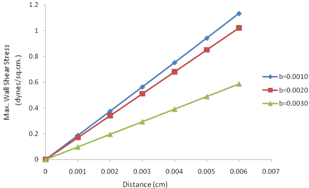
Figure 5(b). Effect of semi-minor axis on the maximum wall shear stress in the elliptical canal
