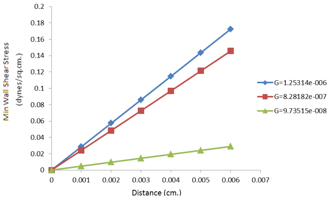
Figure 4(a). Effect of filtration constant on the minimum wall shear stress in the elliptic canal
