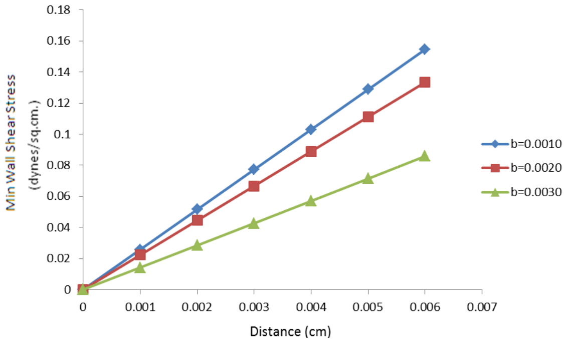
Figure 5(a). Effect of semi-minor axis on the minimum wall shear stress in the elliptical canal
