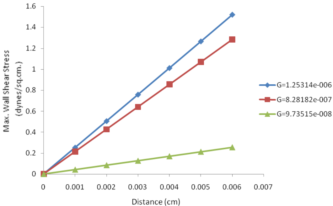
Figure 4(b). Effect of filtration constant on the maximum wall shear stress in the elliptic canal
