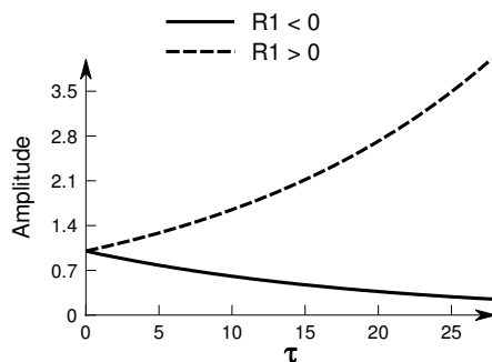
Fig. 4: Amplitude, solution of the equation (44).
