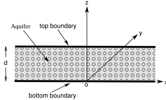
Fig. 1: A schematic diagram for the aquifer problem.
