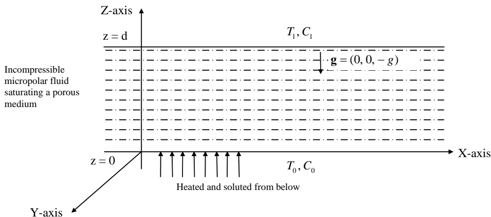
Figure 1. Geometrical configuration
